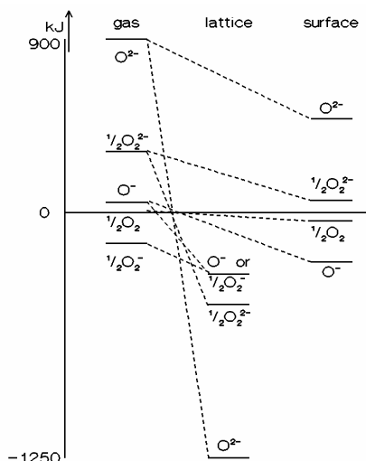
Figure 8. Survey of oxygen species (reproduced from figure 20 of reference 1, copyright 1992, with permission from Elsevier Science).
