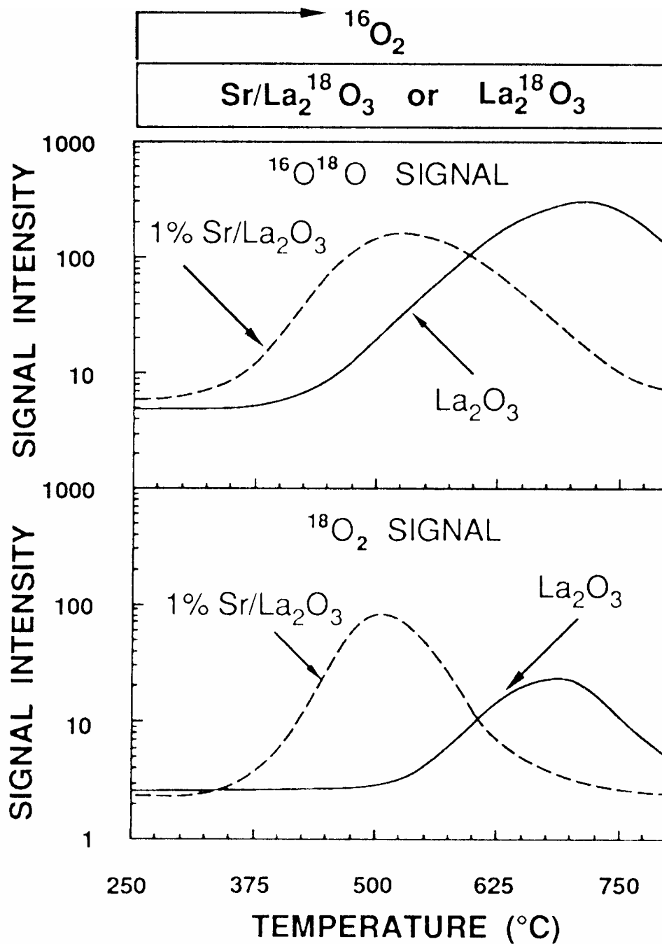
Figure 17. The effect of Sr-promotion on the starting exchange temperature, during a TPIE-experiment (reproduced from figure 5 of reference 112, copyright 1992, with permission from Elsevier Science).
