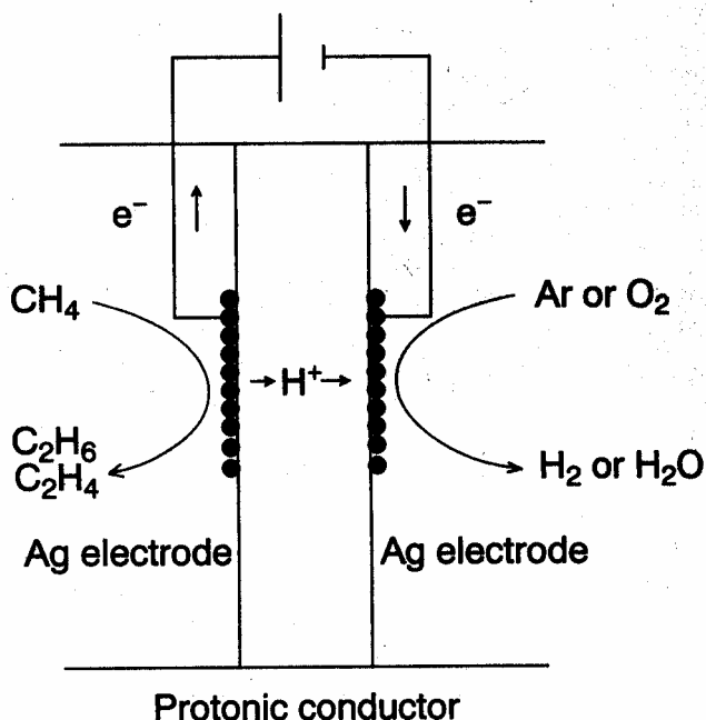
Figure 33. Two compartment cell for the dehydrogenative dimerization of \text{CH}_4 using Ag-electrodes and \text{SrCe}_{0.95}\text{Yb}_{0.05}\text{O}_{3-\alpha} as a solid electrolyte (reproduced from figure 1 of reference 251, copyright 1993, with permission from the The Electrochemical Society, Inc.).
