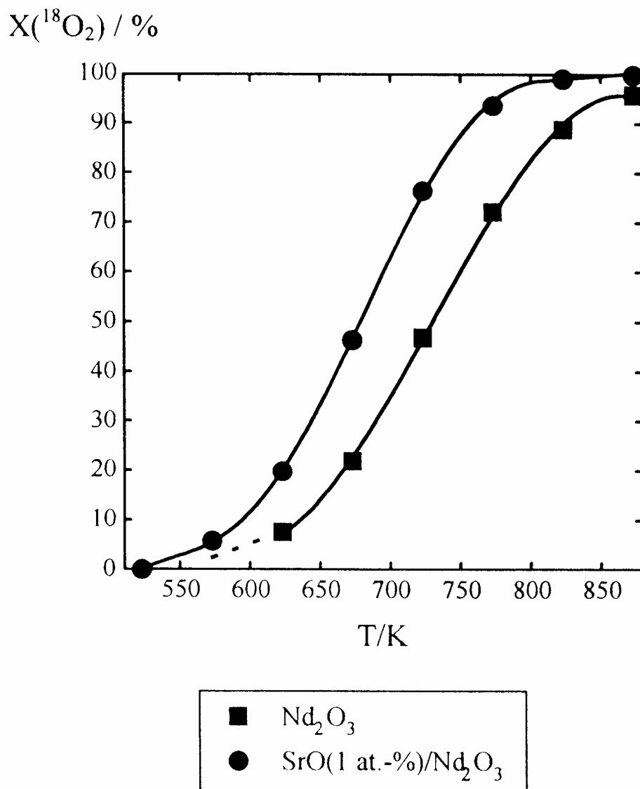
Figure 18. Conversion of ^{18}\text{O}_2 in ^{18}\text{O}^{16}\text{O} by oxygen exchange on \text{Nd}_2\text{O}_3 and \text{SrO}(1 \text{ at.-%})/\text{Nd}_2\text{O}_3 as a function of temperature (reproduced from figure 8 of reference 125, copyright 1998, with permission from Academic Press).
