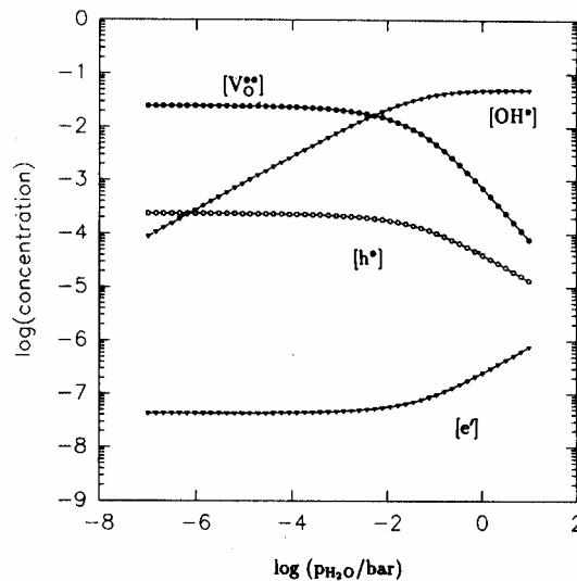
Figure 4. Calculated Kröger-Vink diagram at T = 700\text{ }^{\circ}\text{C} and p_{\text{O}_2} = 0.2\text{ bar} for \text{SrCe}_{0.95}\text{Yb}_{0.05}\text{O}_{3-\alpha} showing the dependence of the concentrations of the four dominant defect types on p_{\text{H}_2\text{O}} (reproduced from figure 5 of reference 18, copyright 1996, with permission from Elsevier Science).
