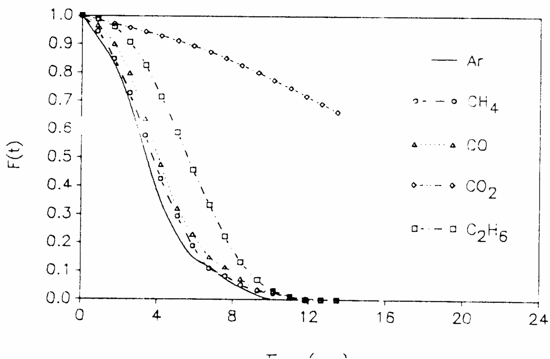
Figure 22. Carbon transients over 32.6 mg Li/MgO at 645 °C (reproduced from figure 6 of reference 127, copyright 1991, with permission from Academic Press).
