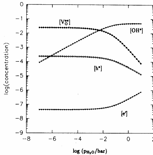
Figure 4. These diagrams, combined with the values of the mobility of the different effects, give more insight into the relative importance and significance of proton contributions to the conductivity.
