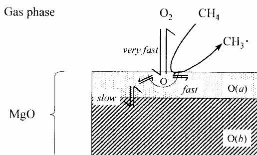
Figure 19. Model of oxygen atom flux in MgO-based catalysts (reproduced from figure 14 of reference 128, copyright 1997, with permission from Academic Press).
