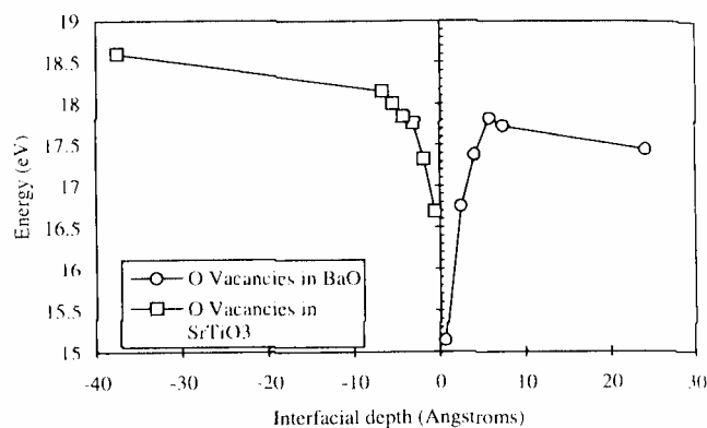
Figure 11 shows the oxygen vacancy formation energies in this system.
