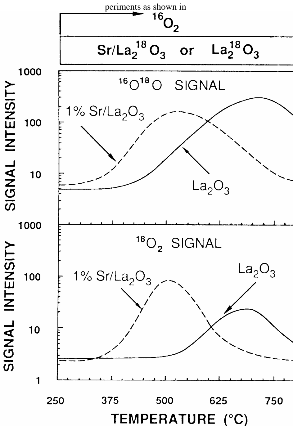
Figure 17 where the ^{16}\text{O}^{18}\text{O} -signal is plotted for both catalysts as a function of the increasing temperature during the experiment. The oxygen exchange starts at a temperature about 100 °C lower for the 1 at% SrO / La 2 O 3 catalyst than for the undoped La 2 O 3 . Also this start lies about 350 °C lower than the usual temperatures used in the oxidative coupling of methane. The results indicate that doping with Sr enables a much faster exchange of lattice oxygen with oxygen from the gas phase, which probably explains the improved activity of the doped catalyst.
