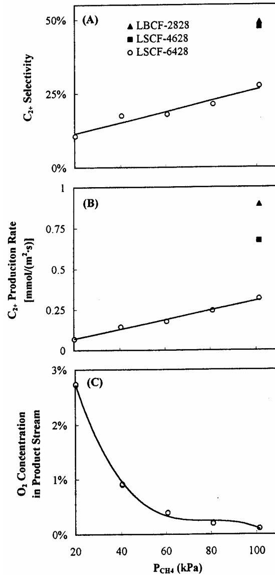
Figure 32. Effect of p_{\text{CH}_4} on methane coupling in a membrane reactor, T = 1098 \text{ K} , p_{\text{O}_2} = 101 \text{ kPa} (reproduced from figure 3 of reference 238, copyright 1997, with permission from the American Institute of Chemical Engineers, all rights reserved).
