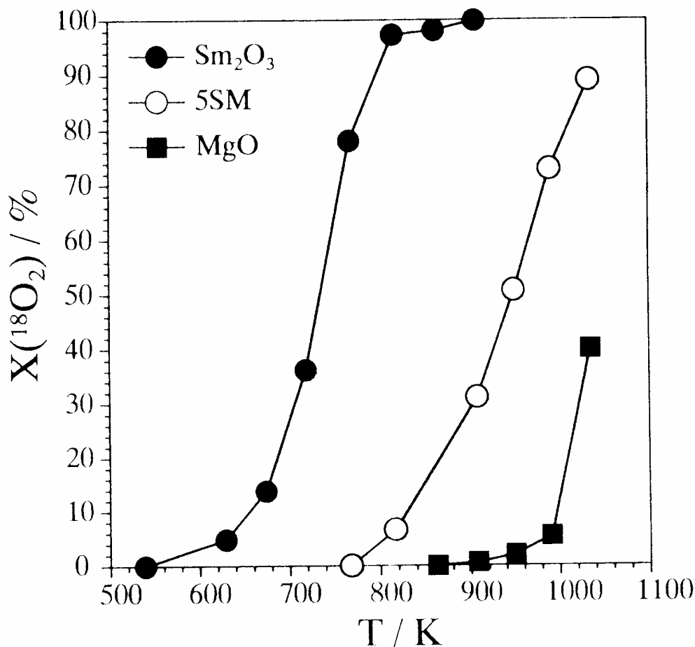
Figure 20. Dependence of the conversion of ^{18}\text{O}_2 in the isotopic exchange reaction on temperature (reproduced from figure 1 of reference 129, copyright 1994, with permission from Academic Press).
