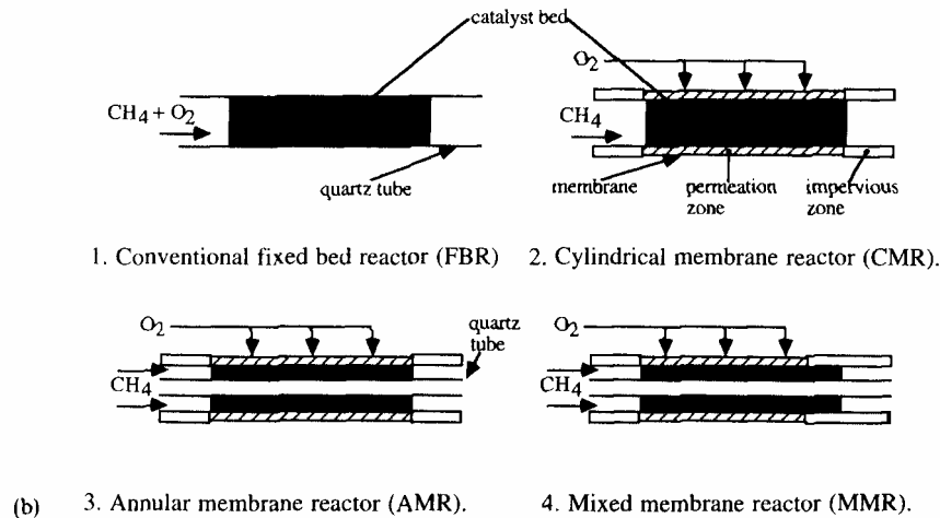
Figure 28. Scheme of different types of reactor configuration. Hatched = porous membrane, black = Li/MgO catalyst (reproduced from figure 1(b) of reference 224, copyright 1994 with permission from Elsevier Science)
