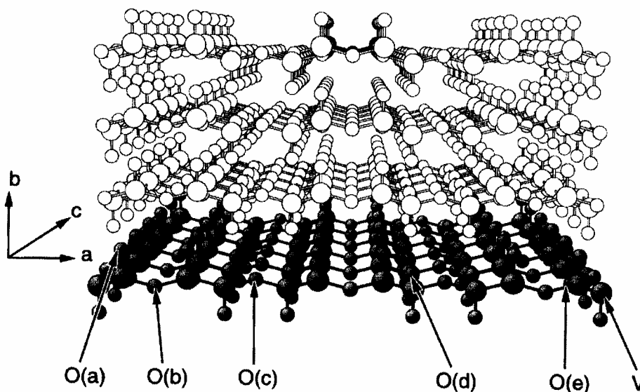
Figure 12. Perspective view of the orthorhombic lattice of V_2O_5 , where the large balls represent V-atoms, the small ones O-atoms. The location of the V-atoms and of the symmetry inequivalent surface O-atoms (O(a)···O(e)) is indicated (reproduced from figure 1 of reference [98], copyright 1997, with permission from Elsevier Science).
