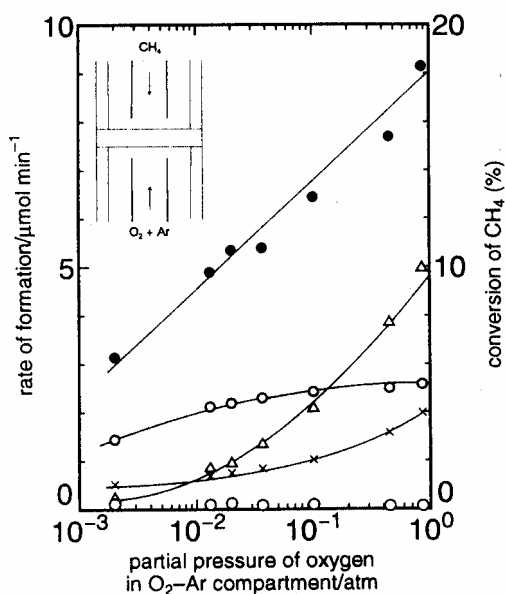
Figure 30. Effect of oxygen partial pressure in O_2 - Ar mixture on formation rates and conversion of methane at 1173 K: \bullet = CH_4 - conversion (reproduced from figure 3 of reference 235, copyright 1997, with permission from the Royal Society of Chemistry)
