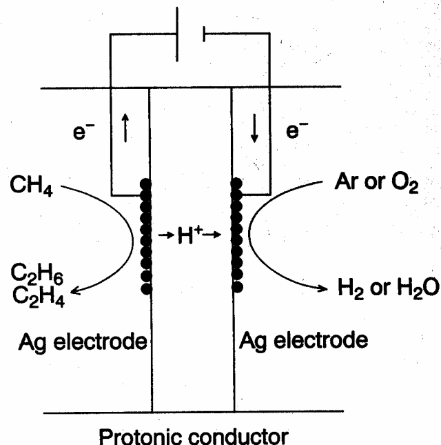
Figure 33. When a current is impressed hydrogen is pumped electrochemically from anode to cathode, enhancing the formation of \text{C}_2 -compounds at the anode. If the electrolyte is not a pure proton-conductor but a mixed proton – electron hole conductor the cell is self-short-circuited and reaction occurs even without external current.
