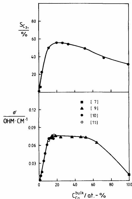
Figure 25. Dependence of C_2 -selectivity and oxygen-ion conductivity on Ca-content of \text{CaO-CeO}_2 catalysts, reaction conditions: T = 1013 \text{ K} , p_{\text{O}_2} = 7 \text{ kPa} , p_{\text{tot}} = 0.1 \text{ MPa} , p_{\text{CH}_4} = 93 \text{ kPa} (reproduced from figure 1 of reference 166, copyright 1992, with permission from Academic Press).
