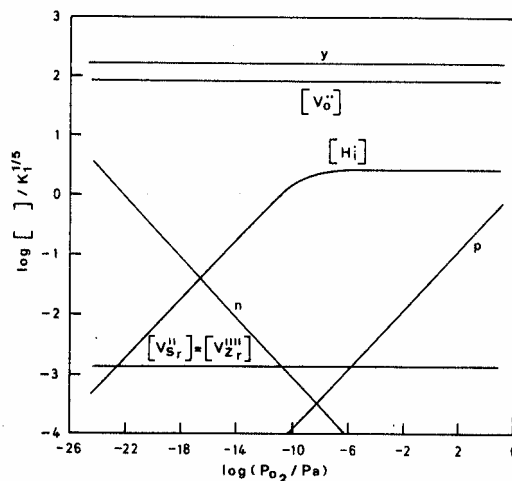
Figure 5. Proposed defect diagram for \text{SrZr}_{0.95}\text{Yb}_{0.05}\text{O}_{3-\alpha} , with y = [\text{Y}'_{\text{Zr}}] (reproduced from figure 5 of reference 24, copyright 1993, with permission from Elsevier Science).
