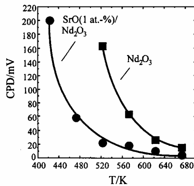
Figure 24. Comparison of change in contact potential difference (CPD) as a function of temperature for Nd 2 O 3 and 1% SrO/Nd 2 O 3 for a change in oxygen partial pressure from 1.0 \times 10^{-3} to 2.0 \times 10^{-3} Pa. (reproduced from figure 6 of reference 125, copyright 1998, with permission from Academic Press).
