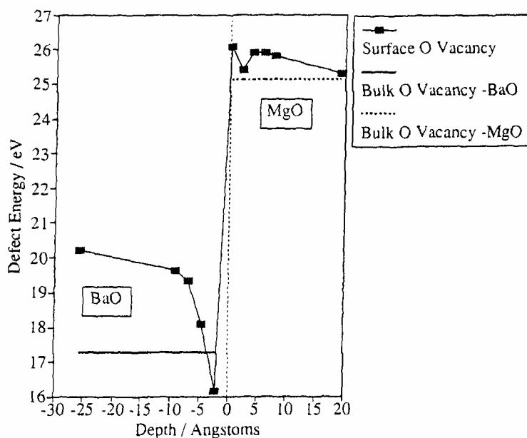
Figure 7. Oxygen vacancy formation energies as a function of depth in the near interface region of the BaO(100)/MgO(100) interface (reproduced with permission from figure 2 of reference 53).
