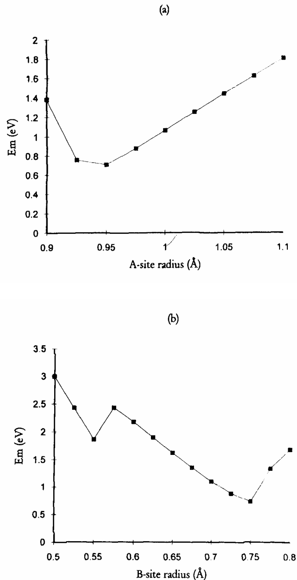
Figure 14. Calculated migration energy as a function of cation size (a) at the A-site (b) at the B-site (reproduced from figure 7 of reference 106, copyright 1995, with permission from Academic Press).
