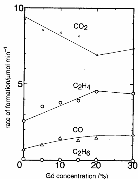
Figure 31. Rates of formation of oxidation products of methane over \text{BaCe}_{1-x}\text{Gd}_x\text{O}_{3-\delta} - powders at 1173 K as a function of \text{Gd}^{3+} -content (reproduced from figure 7 of reference 235, copyright 1995, with permission from the Royal Society of Chemistry).
