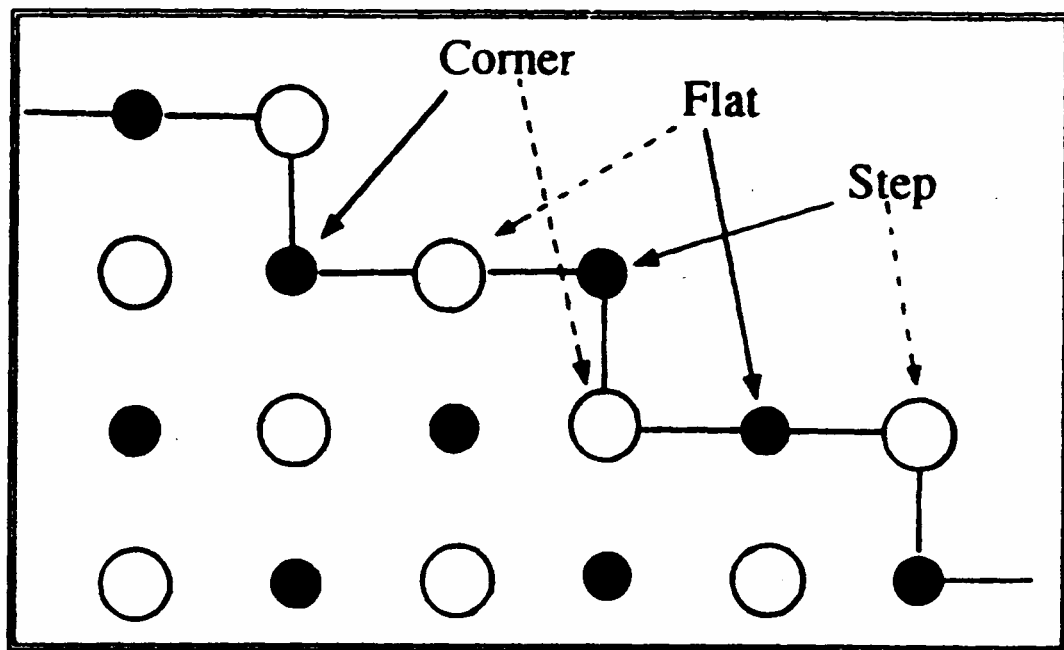
Figure 10. (310) surface plane of \text{CeO}_2 showing three different sites: step, flat and corner. Oxygen: big, open circles, cerium: small, closed circles (reproduced from figure 1 of reference 77, copyright 1994, with permission from Elsevier Science).
