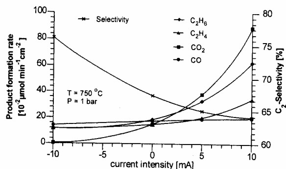
Figure 34. Effect of external current on the product formation rate and \text{C}_2 -selectivity in methane coupling in a membrane cell with SCYO as solid electrolyte (reproduced from figure 11 of reference 255, copyright 1997, with permission from Elsevier Science).
