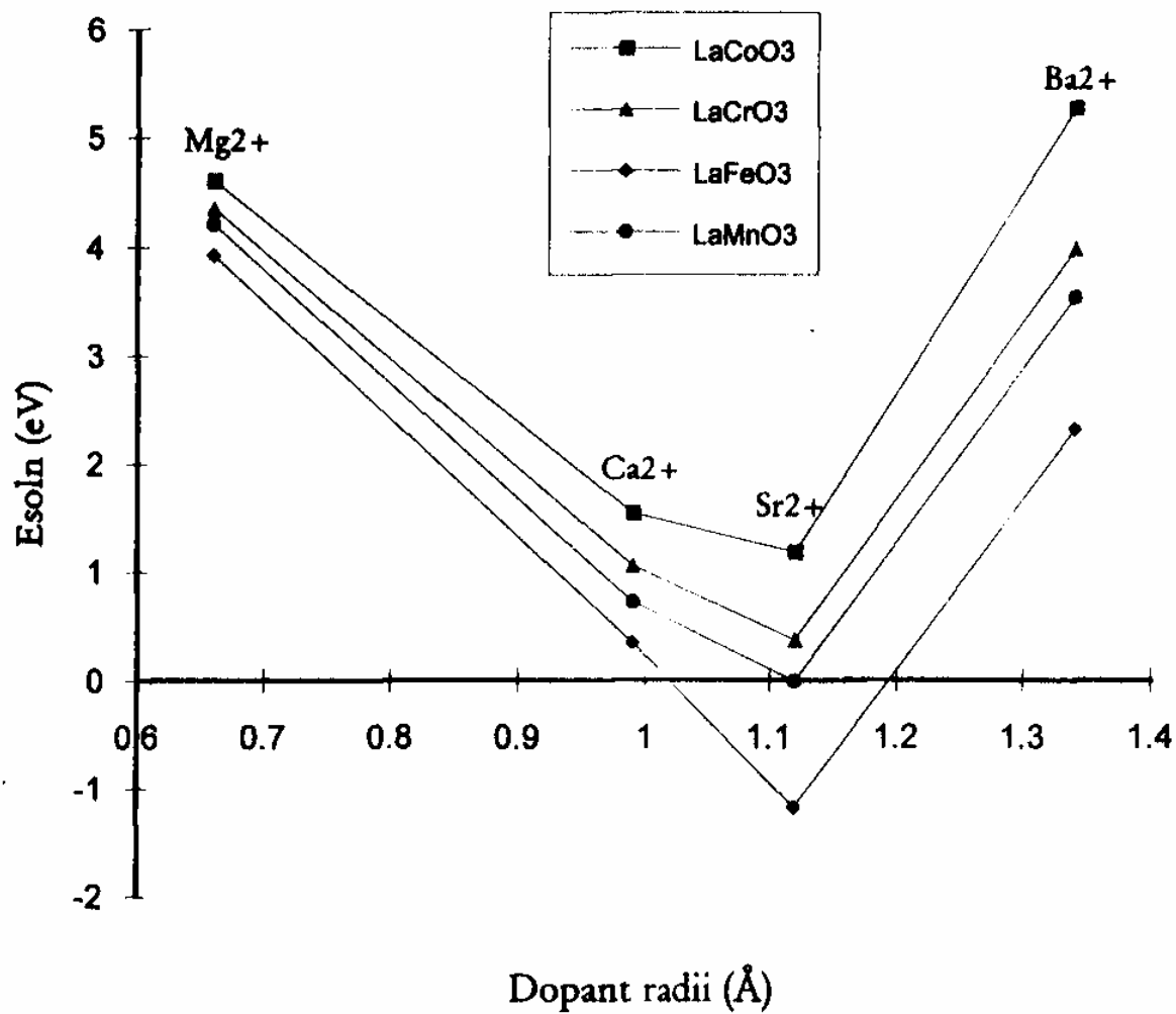
Figure 13. Calculated energies of solution as a function of ionic radius for alkaline-earth dopants in perovskites LaMO_3 , with M = Co, Cr, Fe and Mn (reproduced from figure 9 of reference 106, copyright 1995, with permission from Academic Press).
