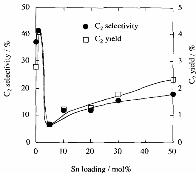
Figure 23. Dependence of C 2 -selectivity and C 2 -yield on tin loading of Sn x – Li/MgO catalysts at 923 K (reproduced from figure 2 of reference 150, copyright 1993, with permission from Academic Press).
