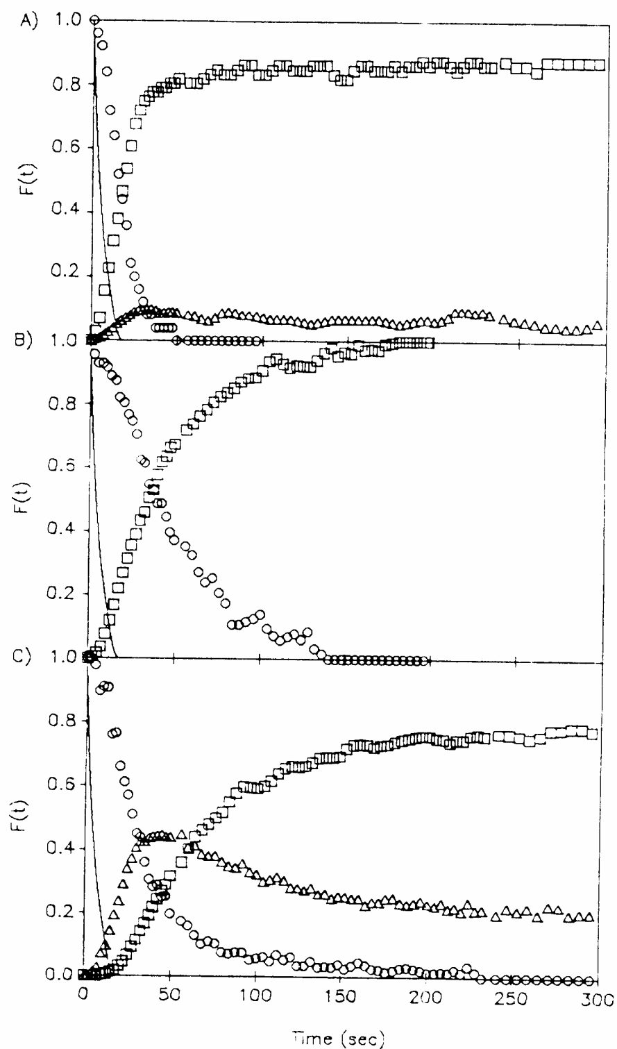
Figure 21. Molecular oxygen transients during reaction with methane at 645 °C over 32.6 mg Li/MgO. A) O 2 – transients, B) CO – transients, C) CO 2 – transients (reproduced from figure 3 of reference 127, copyright 1991, with permission from Academic Press).
