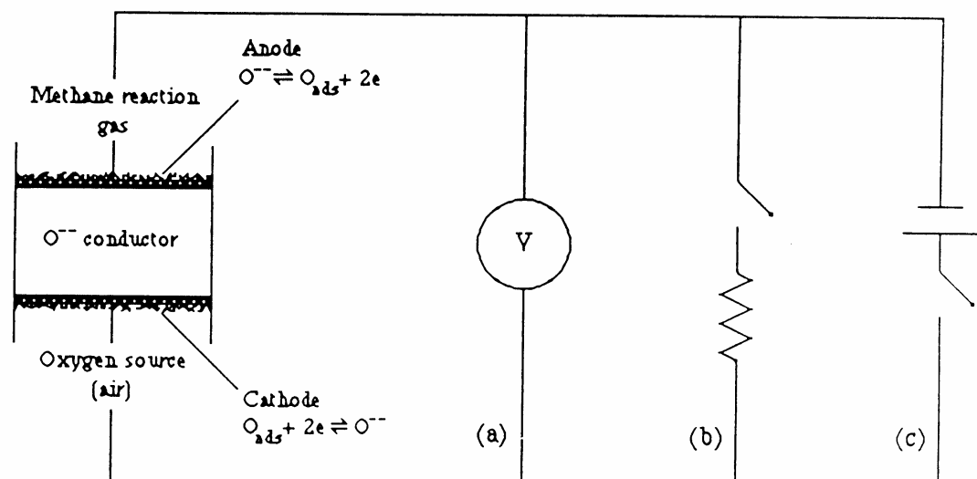
Figure 27. Schematic diagram of solid electrolyte membrane cell with applications: a) open-circuit
