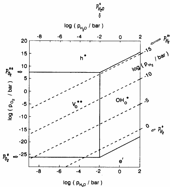
Figure 2. Predominance diagram in the p_{H_2O} - p_{O_2} - plane showing the regions in which the different defects predominate (reproduced from figure 1 of reference 18, copyright 1996, with permission from Elsevier Science).
