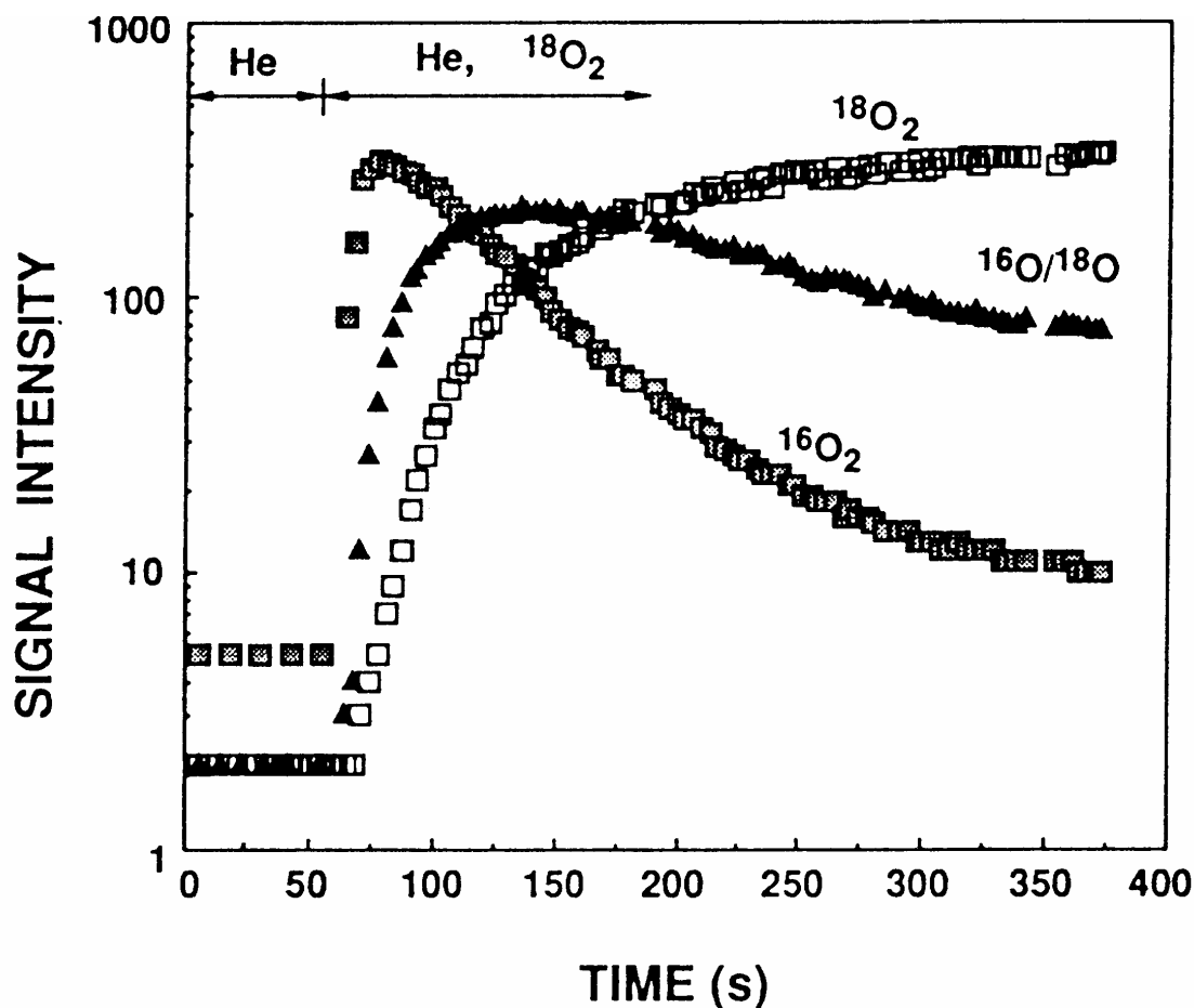
Figure 16. ^{18}\text{O} / ^{16}\text{O} – exchange on 1 at% SrO / \text{La}_2\text{O}_3 catalyst at 750 °C (reproduced from figure 2 of reference 110, copyright 1991, with permission from Baltzer Science Publishers).
