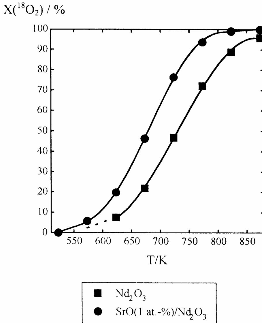
Figure 18. In agreement with the measurements on \text{La}_2\text{O}_3 discussed above here also both the amount exchanged isothermally and the rate of exchange as a function of temperature increase upon doping.
