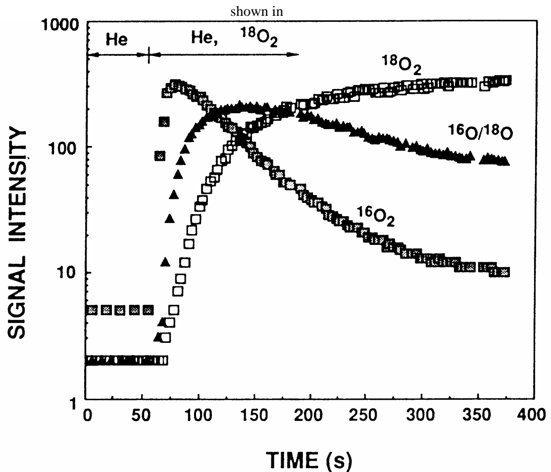
Figure 16. After a time delay corresponding with the reactor dead volume a large amount of ^{16}\text{O}_2 is released from the catalyst, which corresponds with the oxygen adsorbed on and just below the surface. The ^{16}\text{O}^{18}\text{O} -signal behaves differently: it stays constant much longer due to the slow release of ^{18}\text{O} from the bulk of the catalyst. Steady flow of the ^{18}\text{O}_2 is regained after about 5 minutes. For undoped and for 2 at% SrO / \text{La}_2\text{O}_3 similar results were obtained.
